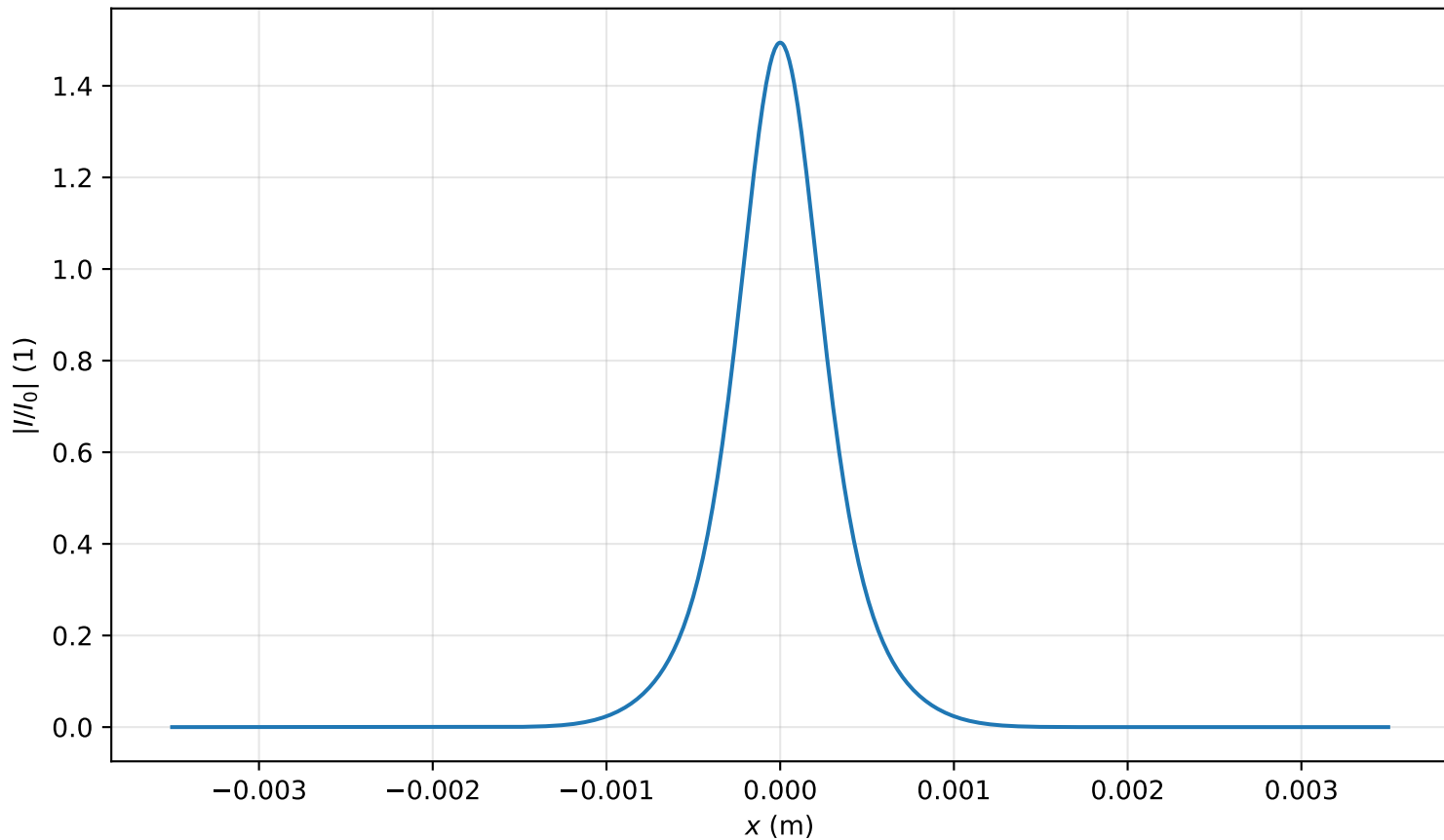
Intensity profile I(x, y = 0, z = 0.955m)/I_0 , P_{in}=1.0P_{cr} , artificial time
